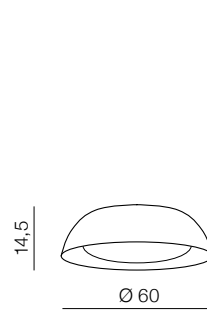
Lenox Top 60 AZ3146 (black/copper) LED 40W 3280lm 3000K aluminium/acrylic
