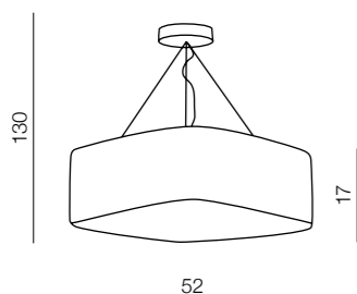
Sugar 52 AZ0448 E27 4x 60W acryl/chrome/clear
