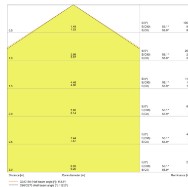
SF BLKH 250 10W/4000K WT IP65
