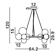
ODILLIA - 9028855 Smoky Grey Glass & Matt Black LED G9 11x5 Watt 230 Volt IP20 Bulb Excluded L: 64.2 W: 52.8 H: 120 cm
