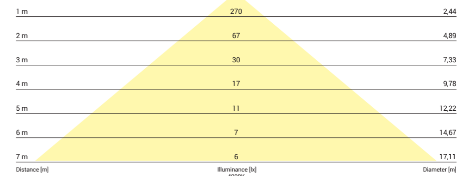
8781, 8W, 4000K, beam angle 100°
