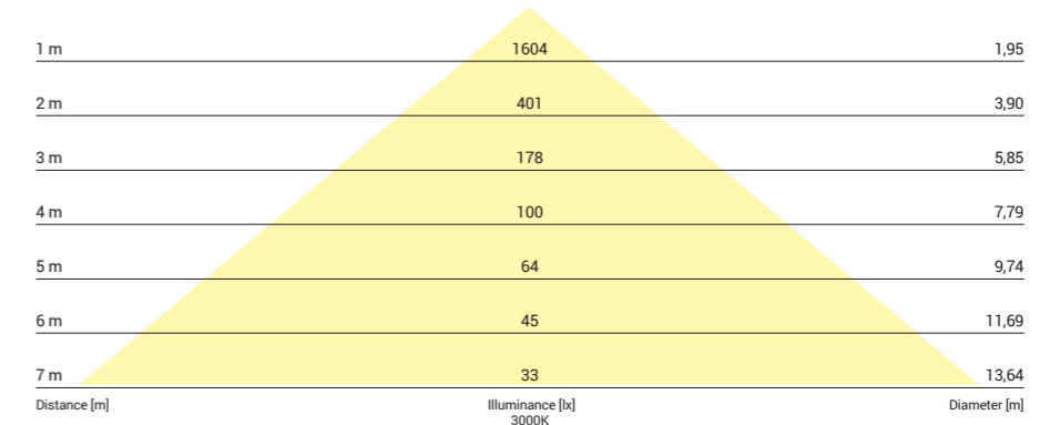
8298, 31W, 3000K, beam angle 90°
