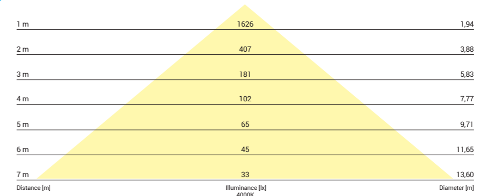
8297, 31W, 4000K, beam angle 90°
