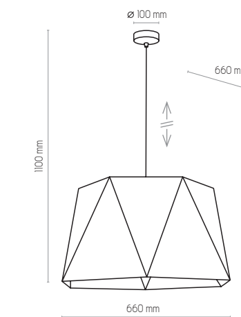
3129 | IVO | 1x E27, 25W LED | AB 9953
