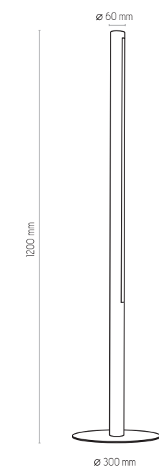
1409 | ROLLO | 1x 230V, 30W, 3000K, 3250lm
