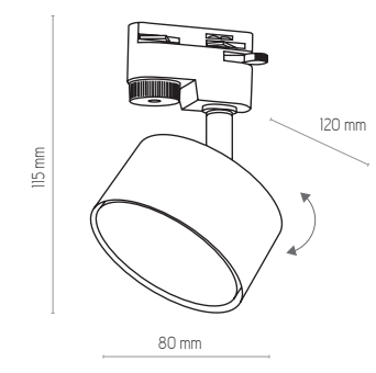
4397, 4398 | TRACER | 1x GX53, 15W LED
